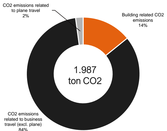
Figuur 3: CO 2 -emissie ANL 2021 per scope
